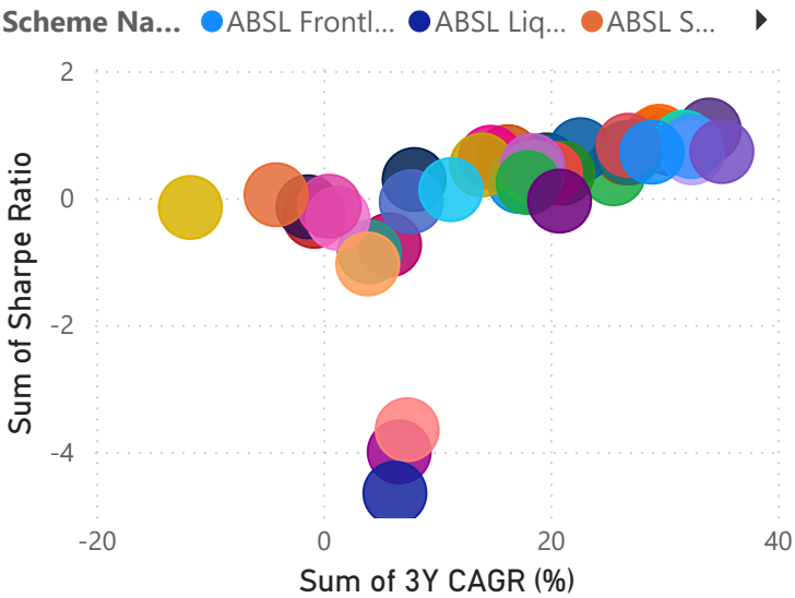
Sum of 3Y CAGR (%), Sum of Sharpe Ratio and Sum of aum_crore by Scheme Name
